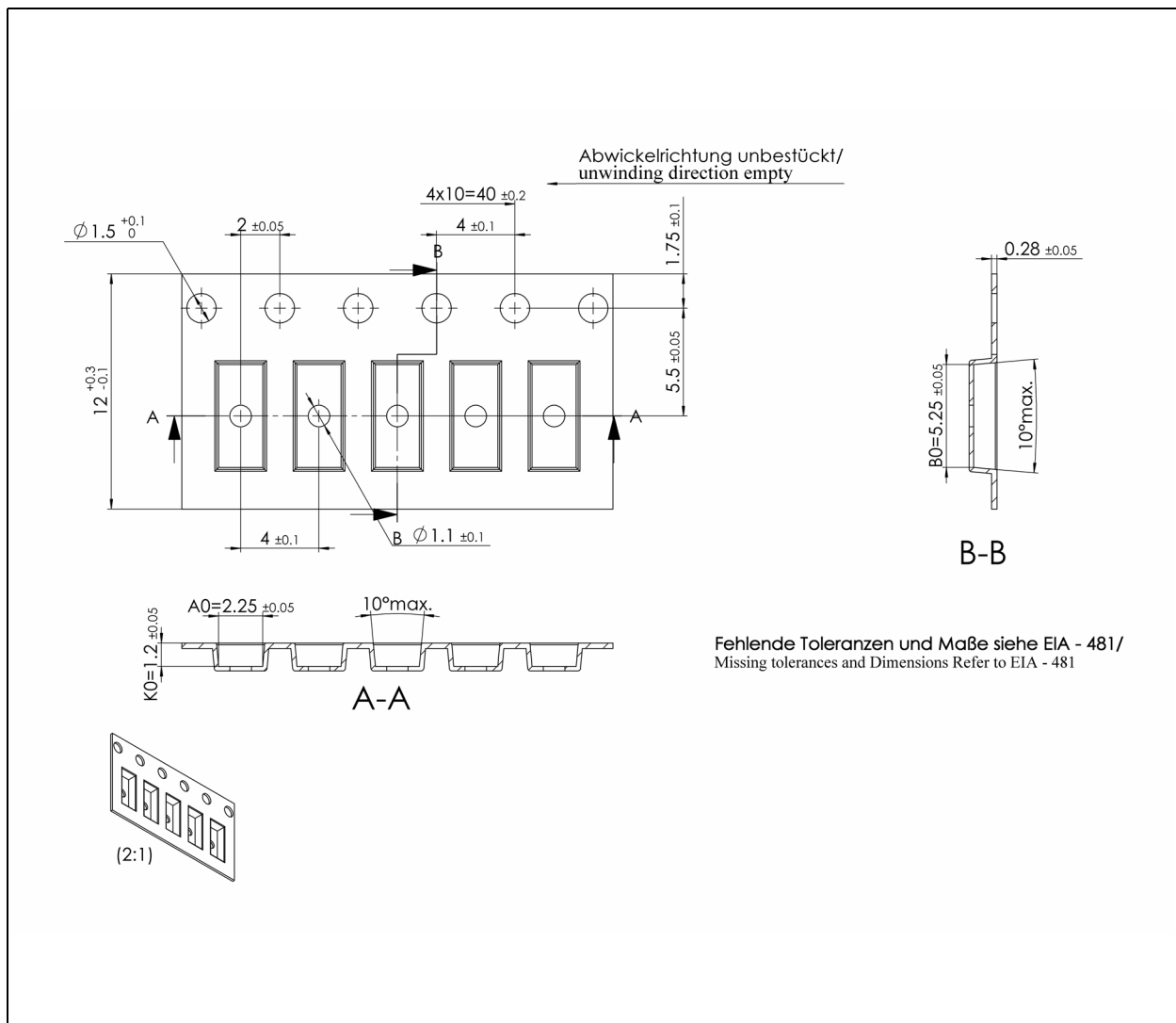
Figure 75: Tape and Reel Mechanical Drawing
